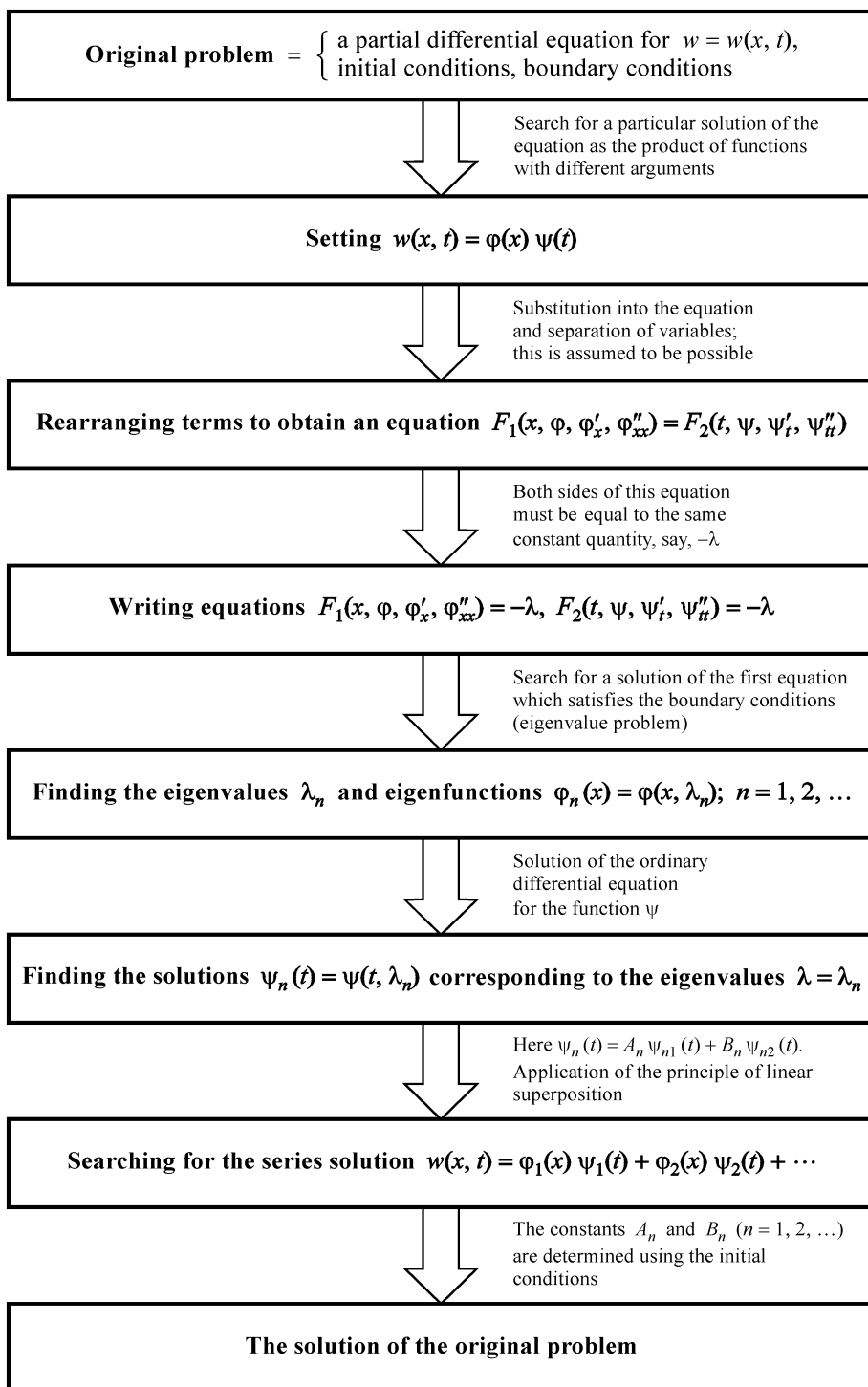
Figure 1. Scheme of solving linear boundary value problems by separation of variables (for parabolic equations, the function F_2 does not depend on \psi''_{tt} , and B_n = 0 ).
