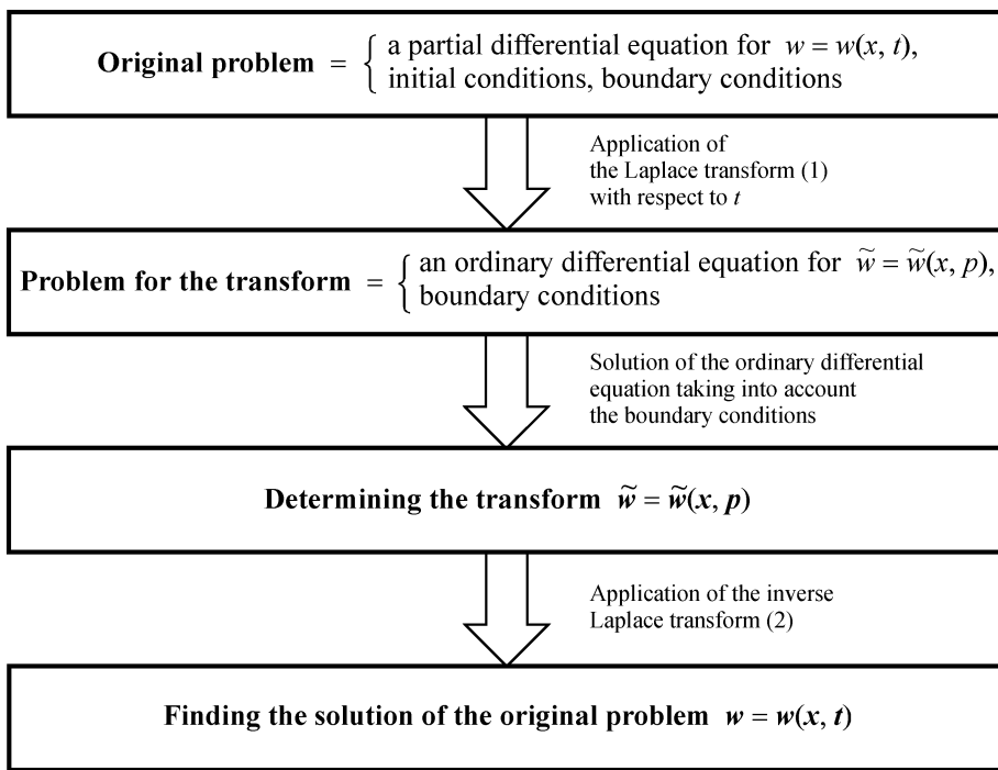
Figure 2. Scheme for solving linear boundary value problems by the Laplace transform.
