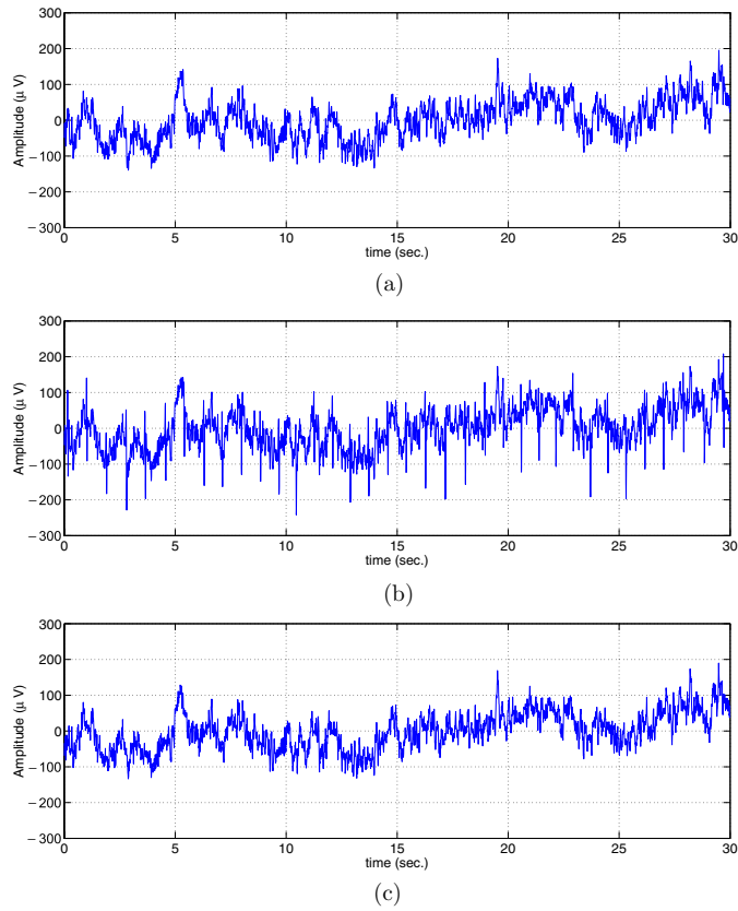
Figure 2. Results of the EKS on a mixture of simulated signal plus ECG artifacts. The (a) original, (b) noisy and (c) denoised signals can be seen in this figure. The SNR of the noisy signal was improved from 7.6 dB to 15.1 dB using the EKS.
