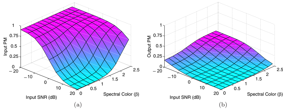
Figure 4. Periodicity measures (PM) achieved on simulated data in different input SNRs and different spectral colors, (a) before and (b) after denoising. The decrease of PM is used as a necessary, but not sufficient, measure of the filtering performance.
