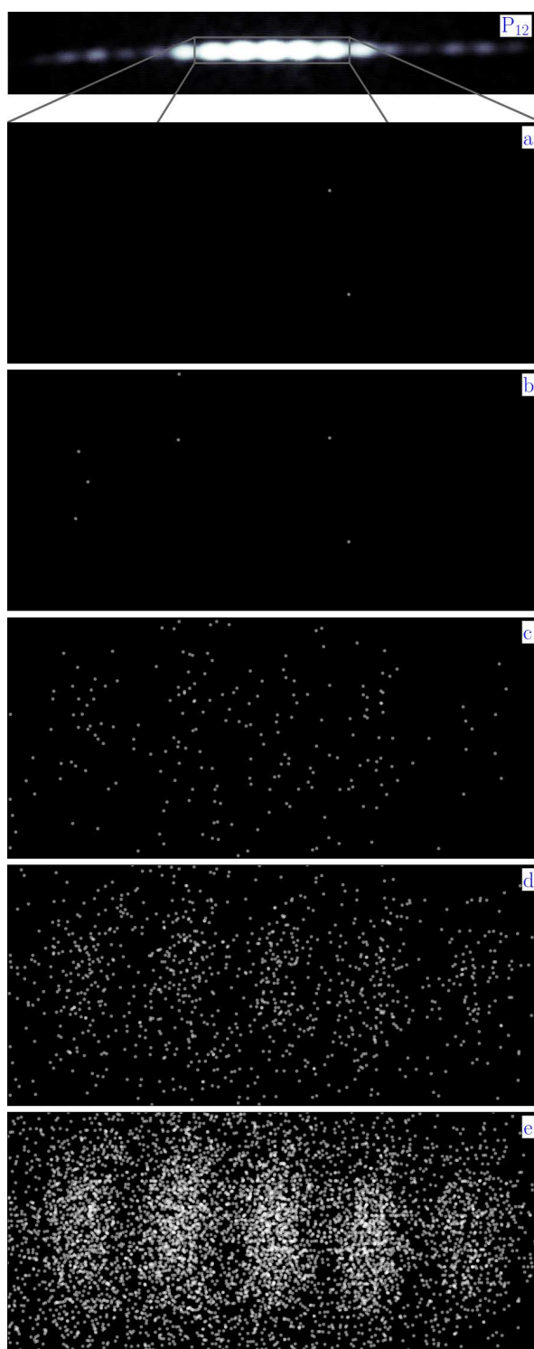
Figure 3. Buildup of electron diffraction. “Blobs” indicate the locations of detected electrons. Shown are intermediate build-up patterns from the central five orders of the diffraction pattern ( P_{12} ) magnified from figure 2, with 2, 7, 209, 1004, and 6235 electrons (a-e). A full movie of the electron build-up is included in the supplementary data (see Supplementary Movie 2)
