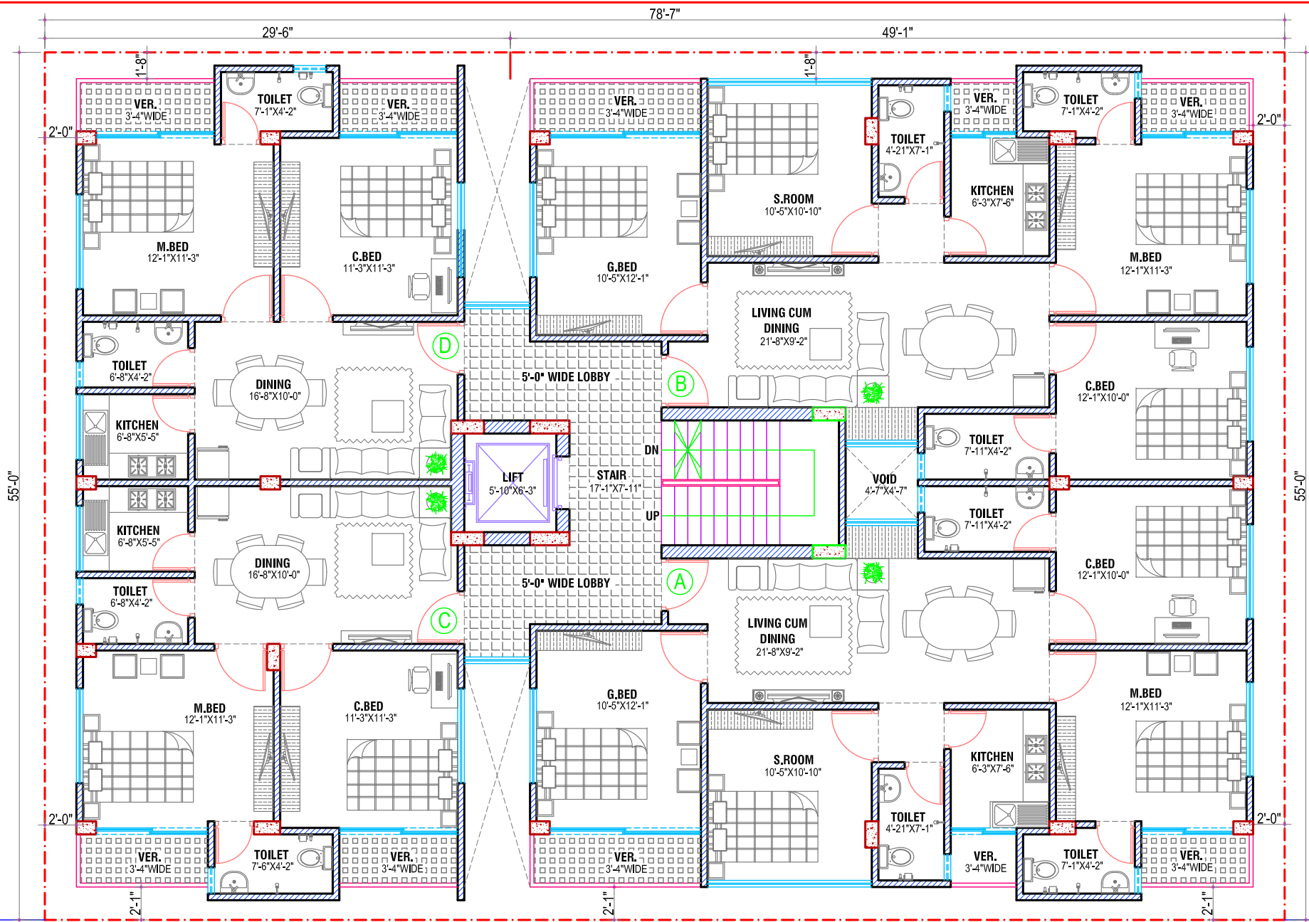
TYPICAL FLOOR LAYOUT PLAN SCALE : 1/8" = 1'-0"
