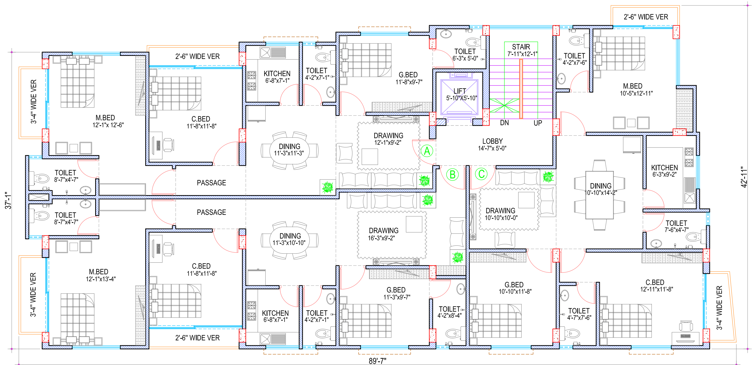
TYPICAL FLOOR LAYOUT PLAN SCALE : 1/8" = 1'-0"
