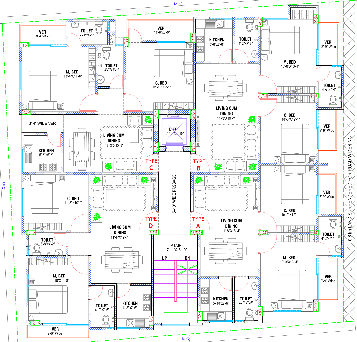
TYPICAL FLOOR LAYOUT PLAN SCALE : 1/8" = 1'-0"
